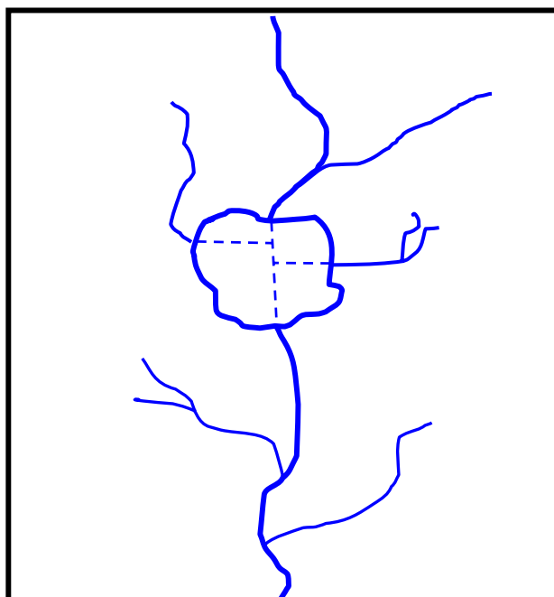
Fig.1. The network is connected manually through the lake. For simple lakes this could be straight lines joining the main channel to the lake tributaries.
