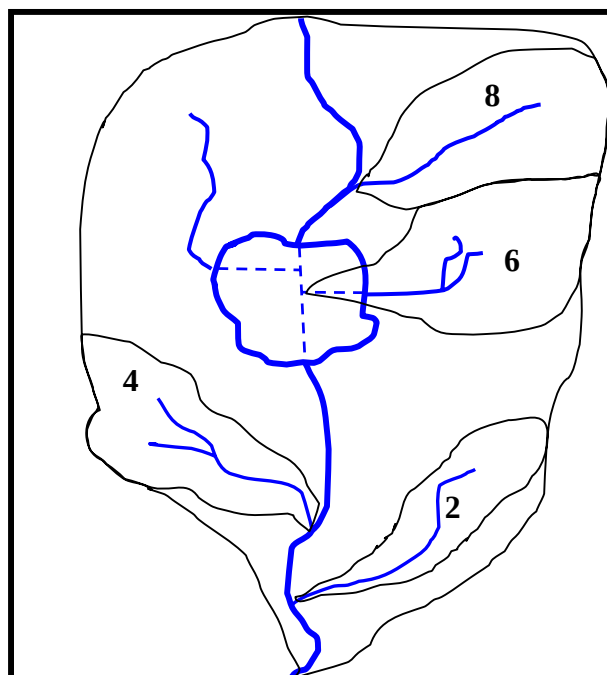
Fig. 2. The major tributaries are identified, while ignoring the presence of the lake.
