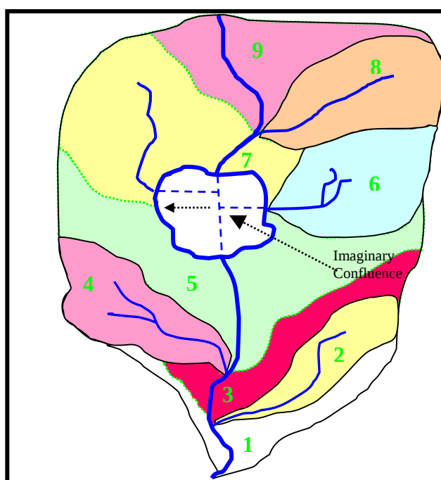
Fig. 4. Alternative approach to tributary catchment 06. Inter-basin boundaries meet the lake at a points determined by elevation model interpolation (e.g. basins 5 and 7).
