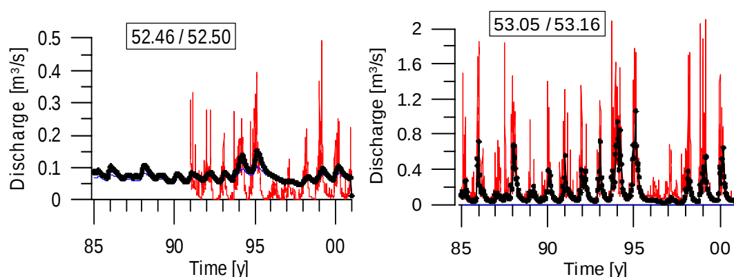
Figure 1: Calibration of hydraulic model on streamflow-data. Thick line: model results. Thin dashed line: recorded discharge. Left a poorly calibrated/determined, and therefore less precise, model. Right a well-calibrated/determined model.
