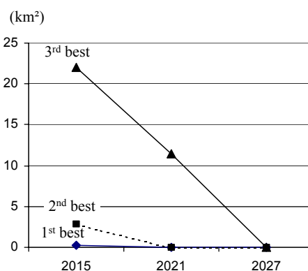
Figure 2: Area where the salt concentration is higher than 250 mg/l for the three scenario (in km²)
