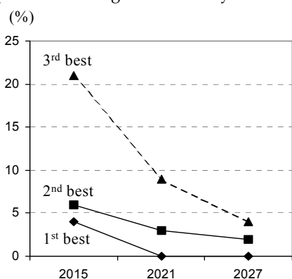
Figure 1: Quantity of salt remaining in the aquifer as a percentage of the initial stock
